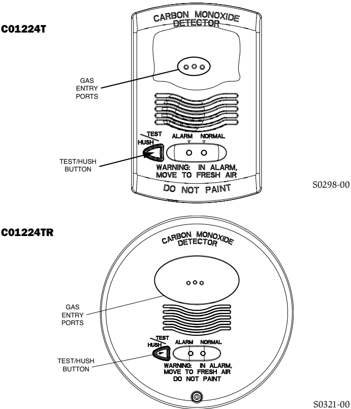
FIGURE 4. TEST BUTTON LOCATION AND OPERATION:
